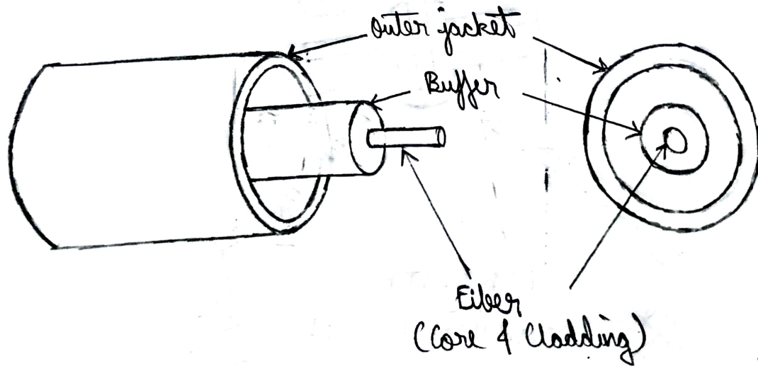
FIBER OPTIC CABLE
